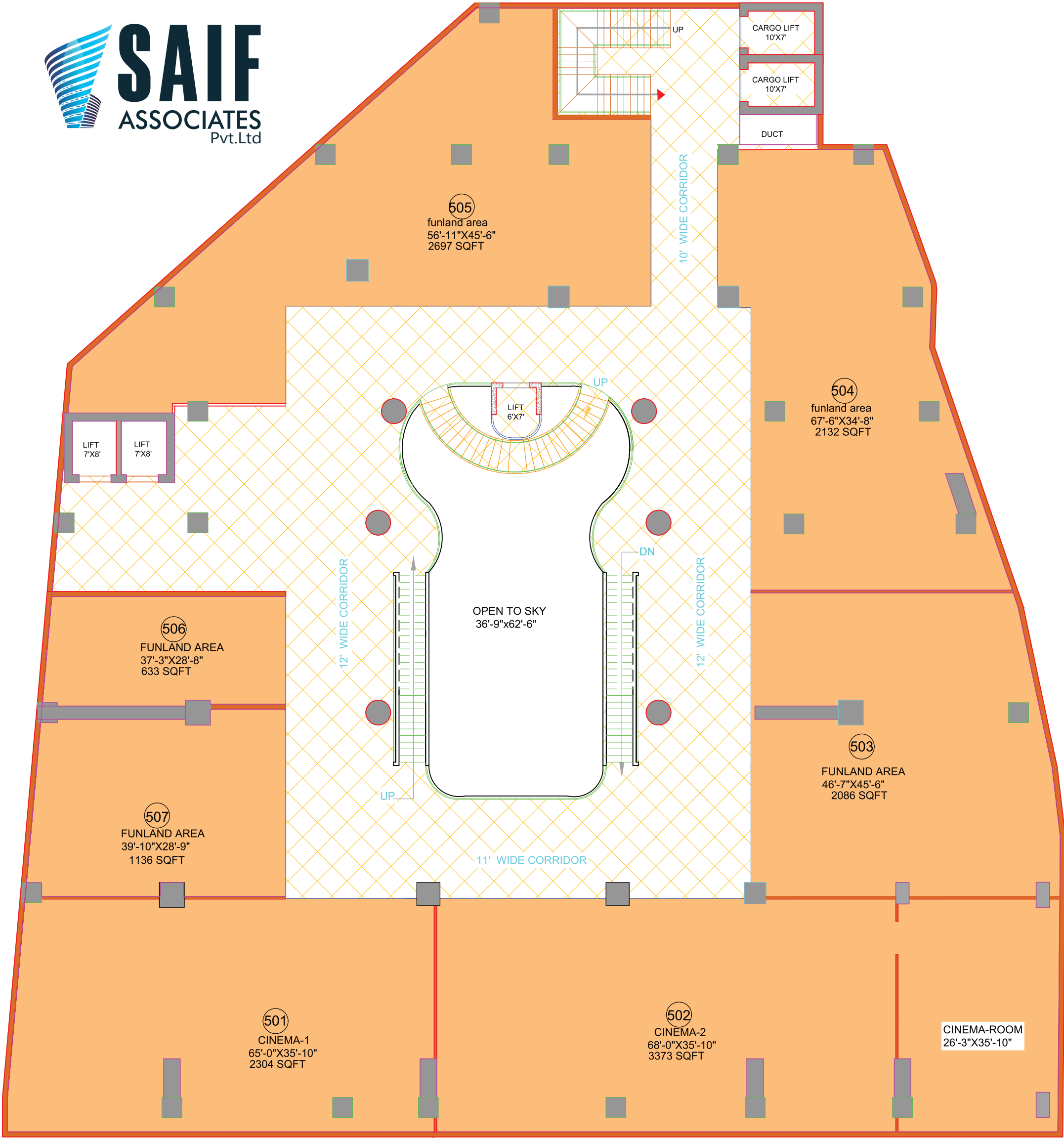
FIFTH FLOOR PLAN
