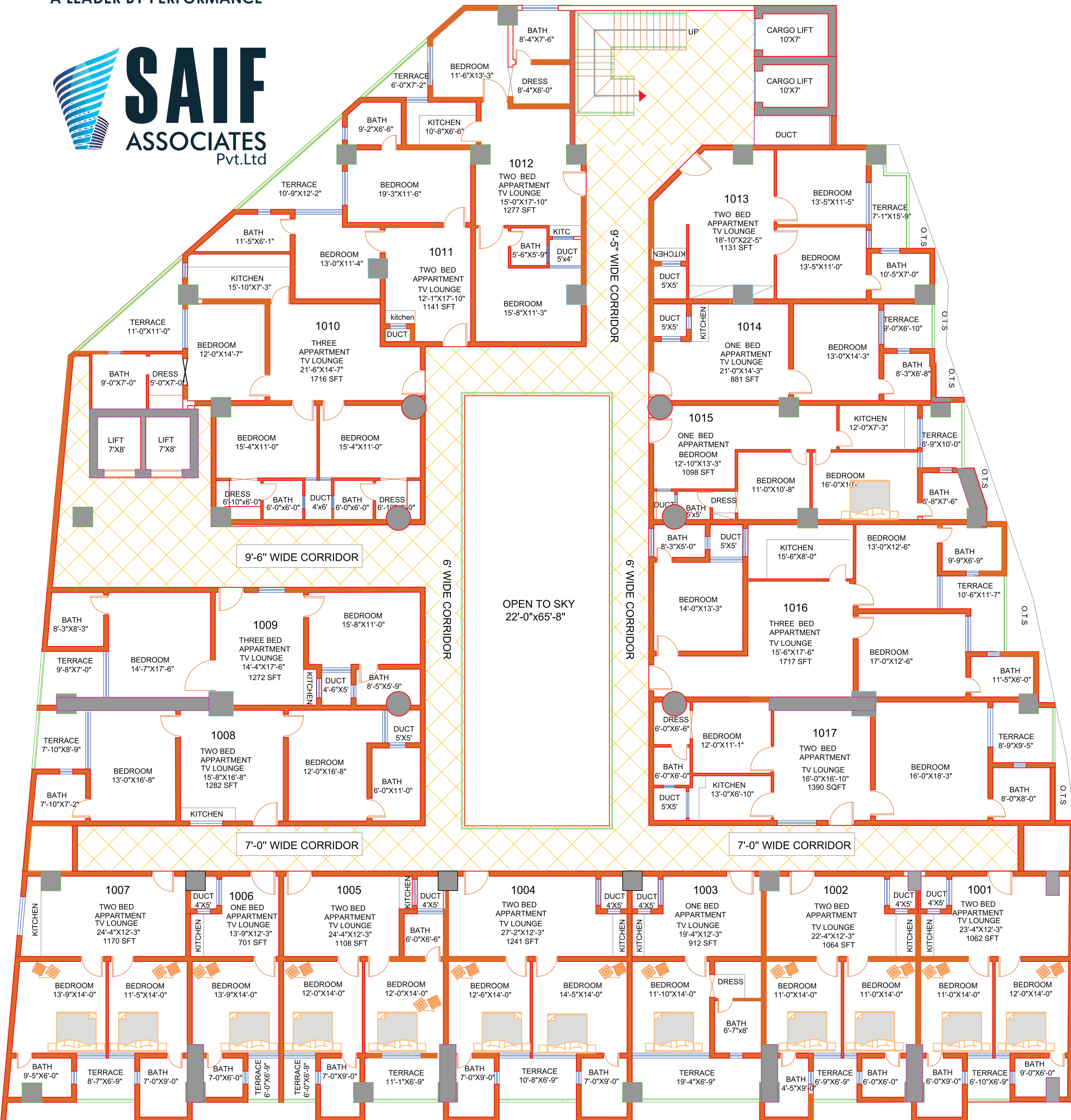
10TH FLOOR PLAN
