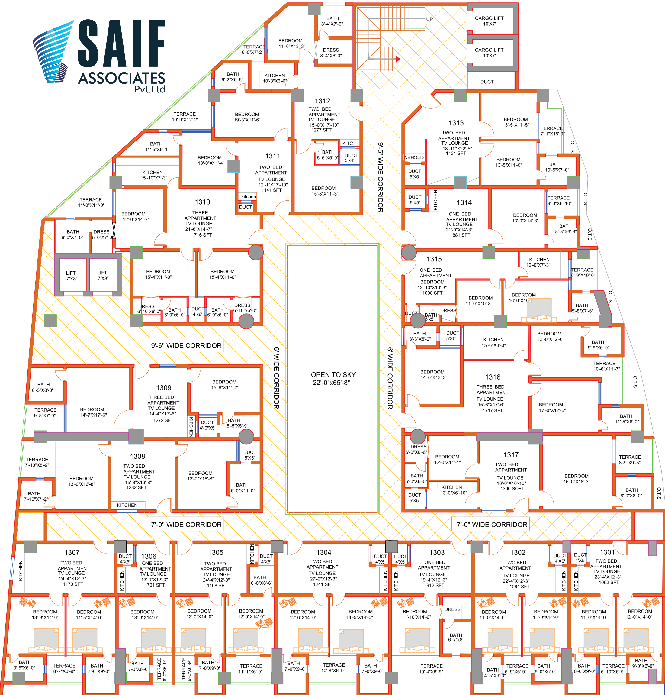
13TH FLOOR PLAN
