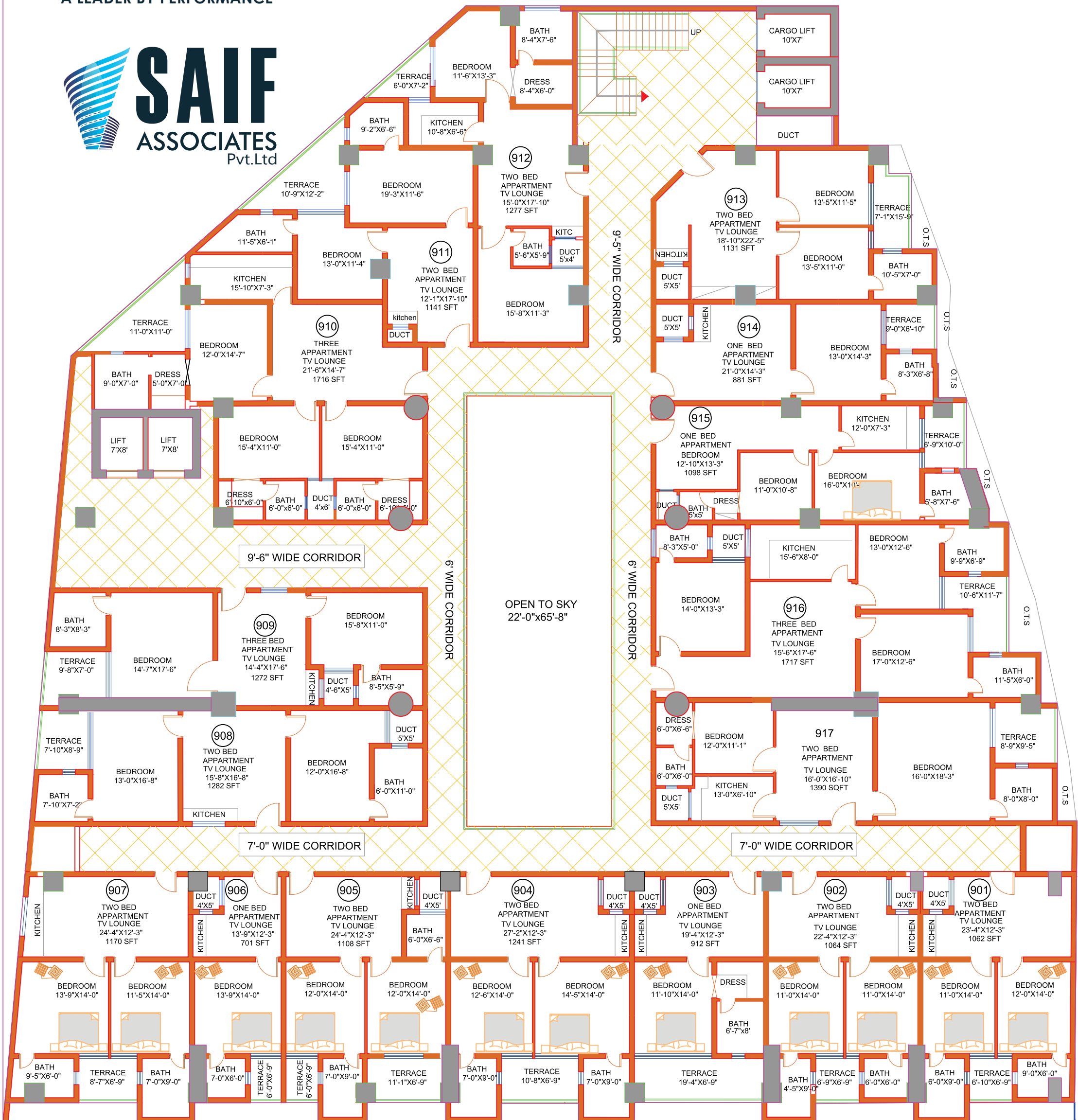
9TH FLOOR PLAN
