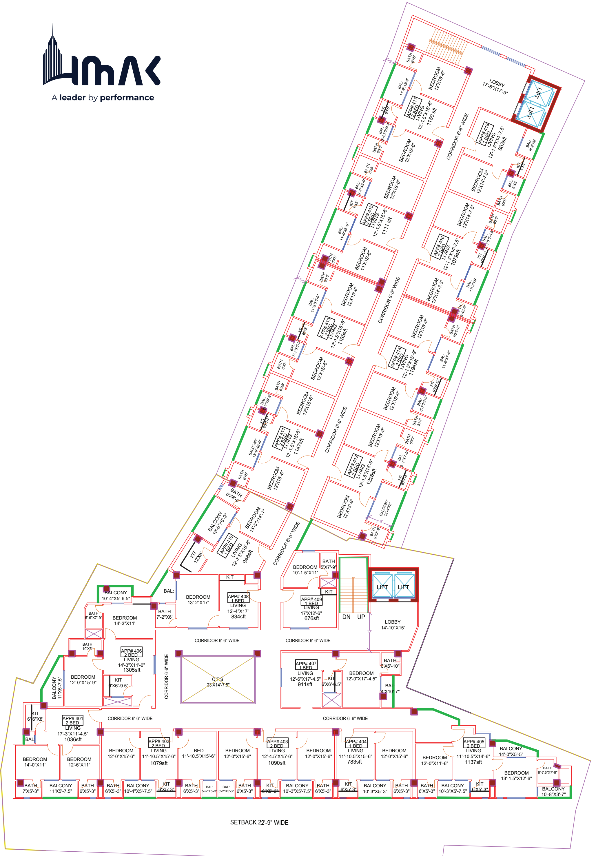
4TH FLOOR PLAN APARTMENTS
