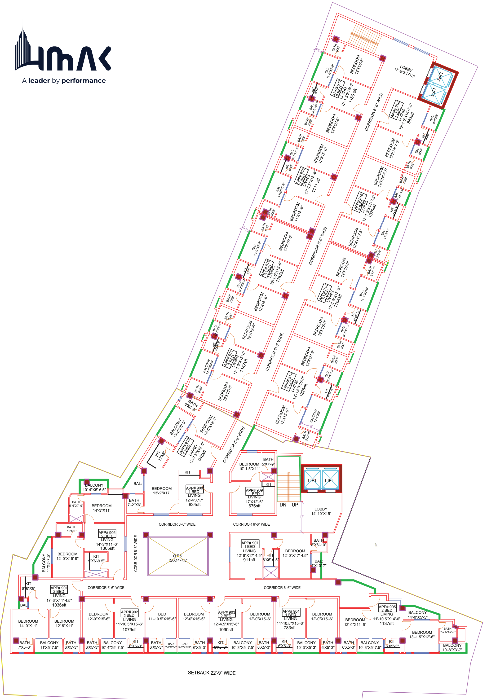
9TH FLOOR PLAN APARTMENTS
