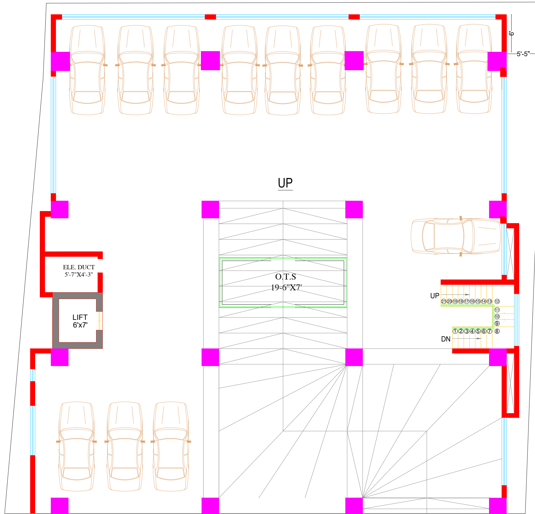
LEVEL -1 FLOOR PLAN COVERED AREA: 5989 SFT
