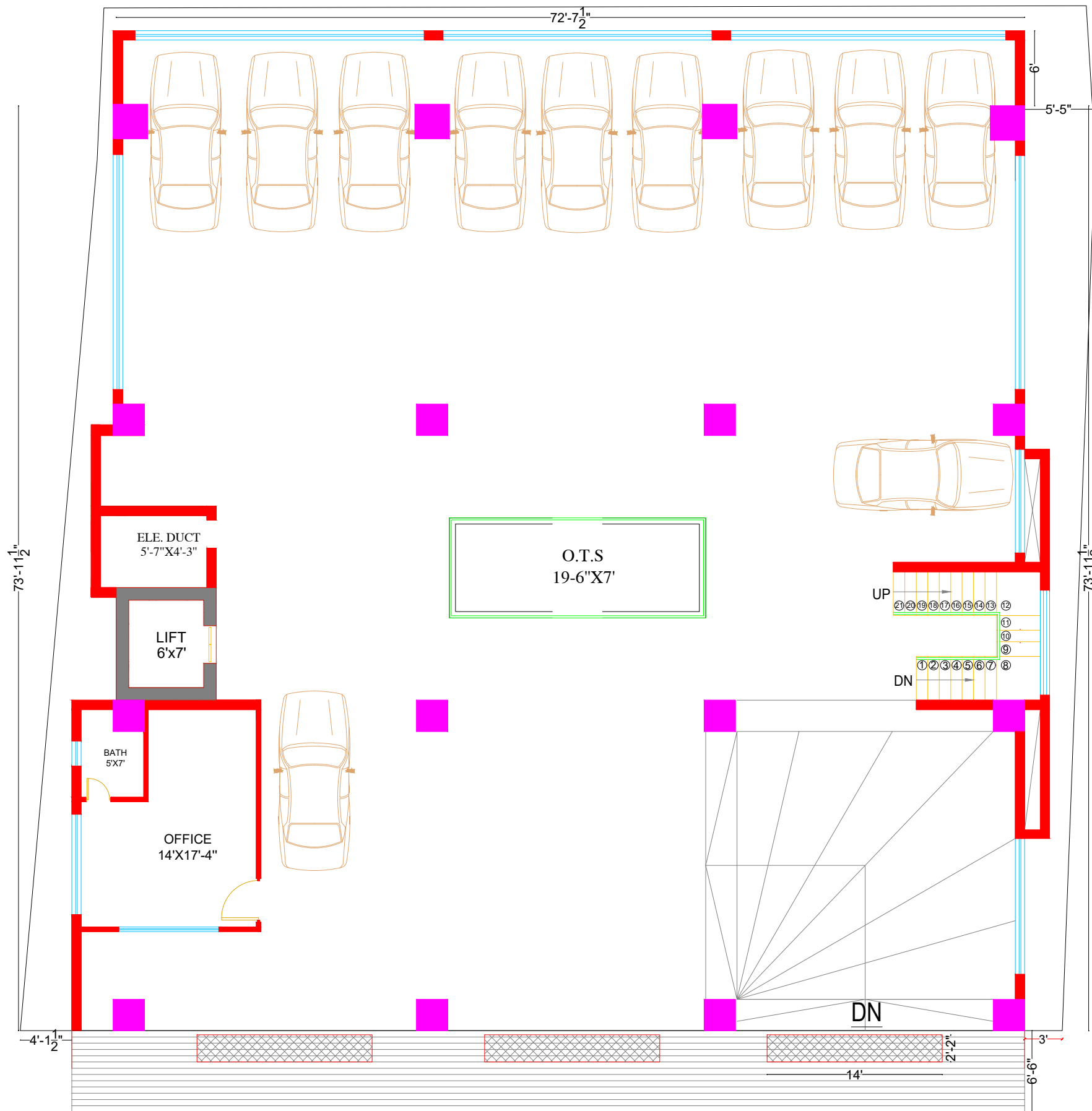
GROUND FLOOR PLAN COVERED AREA: 5989
